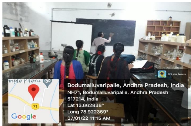
III B.Sc Structure of Glucose
